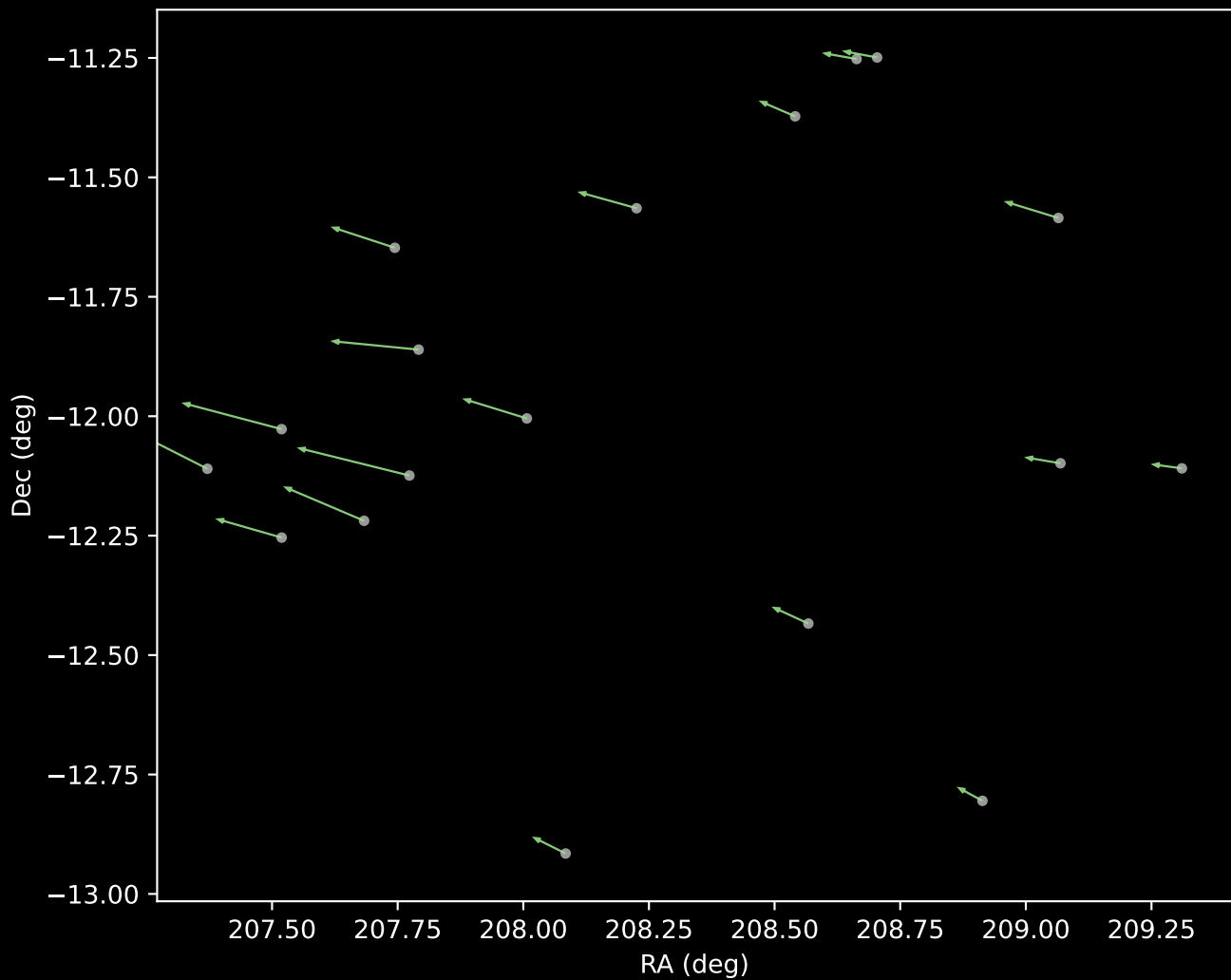
GALAH DR4 Cluster 5 Proper Motion Vectors (n=18)
