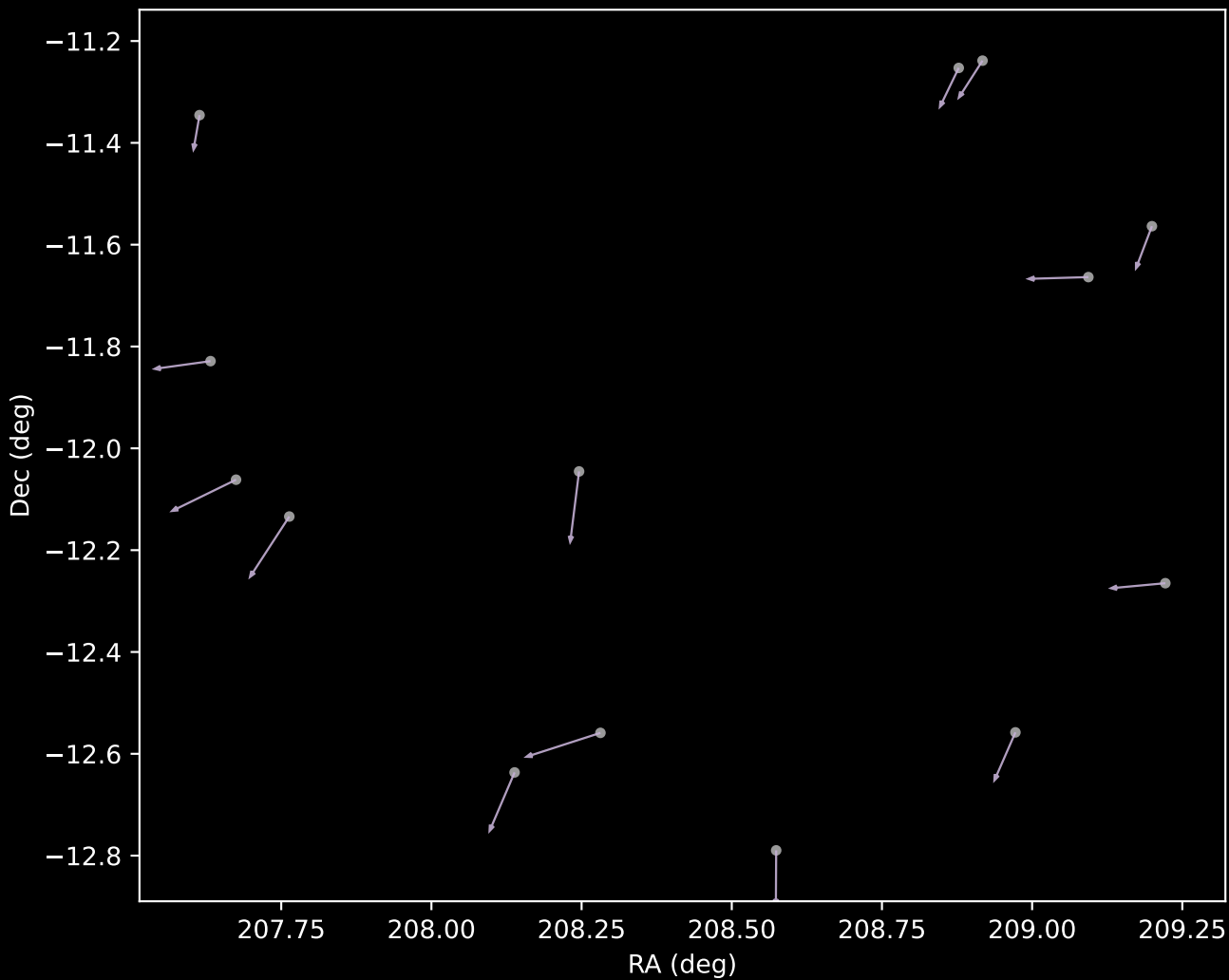
GALAH DR4 Cluster 9 Proper Motion Vectors (n=14)
