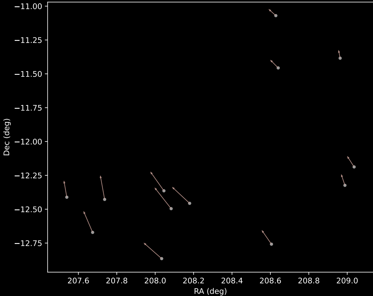
GALAH DR4 Cluster 11 Proper Motion Vectors (n=13)
