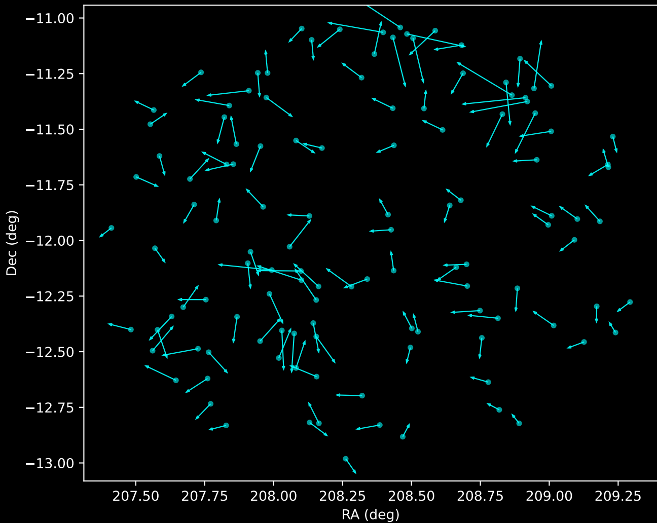
GALAH DR4 Noise Stream Proper Motion Vectors (n=121)
