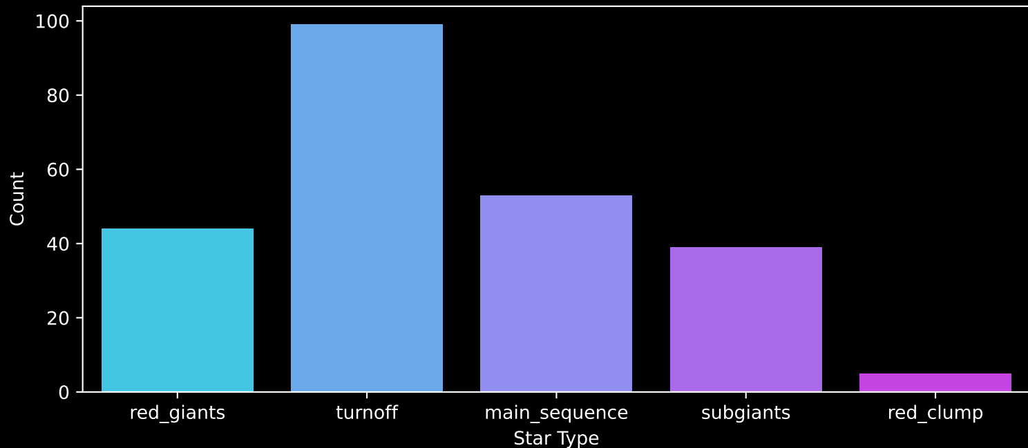
GALAH DR4 Field: [8828] Count plot of Star Type
