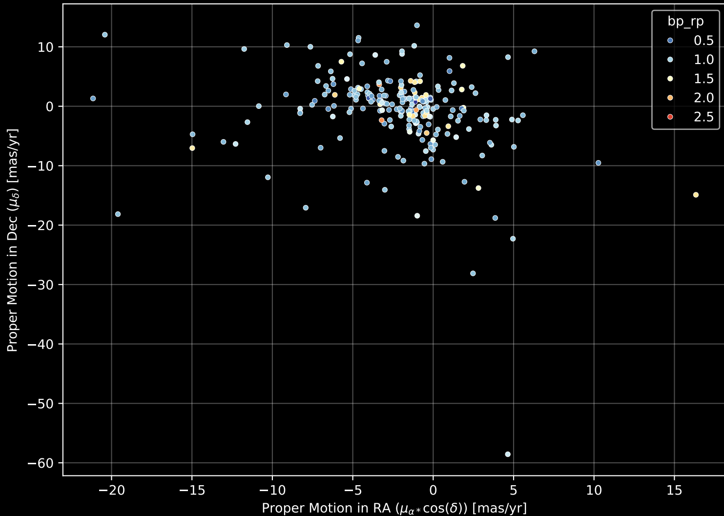
GALAH DR4 Field: [8828] Proper Motion Diagram (n= 240)
